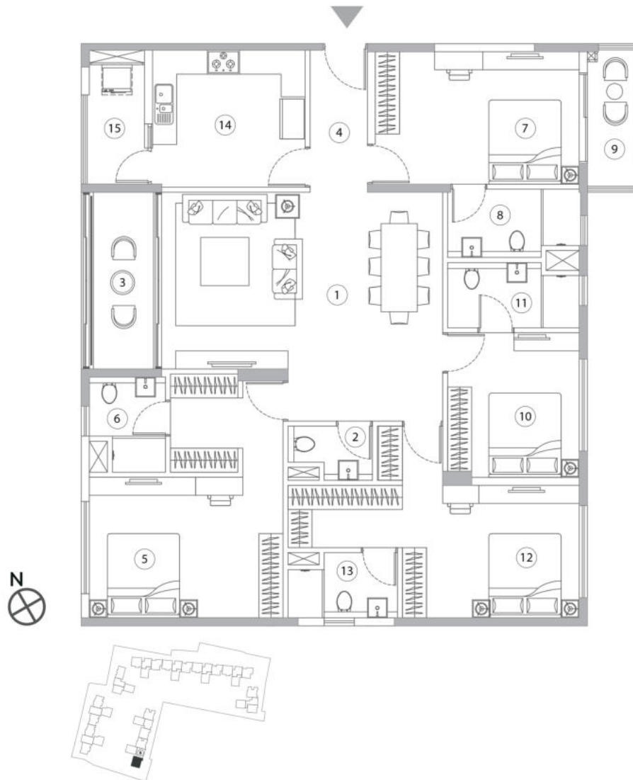
UNIT C SIMPLEX (FLOOR 2 TO 11)
