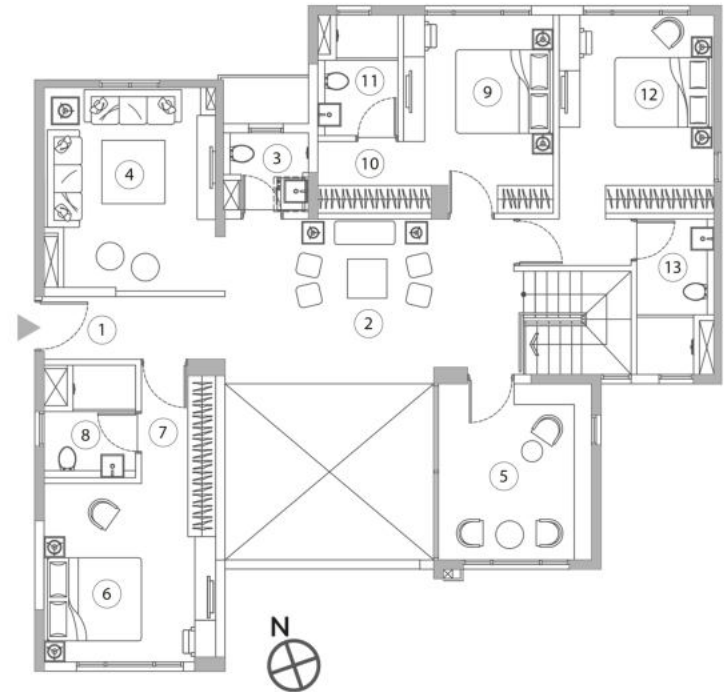
UNIT B DUPLEX UPPER (FLOOR - 2)
